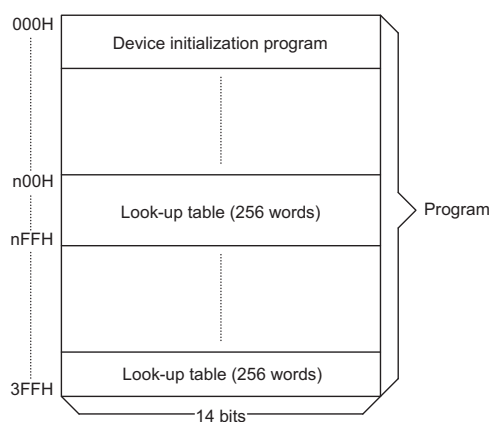
Program Memory
