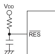
Reset Circuit
