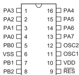
HT48R062/HT48C062 — 16 DIP-A/SOP-A/SSOP-A
