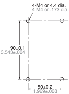
Mounting dimensions
