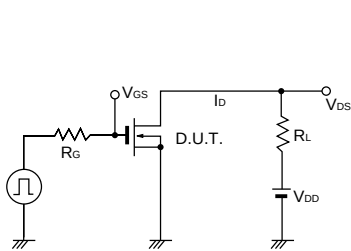
Fig.17 Switching Time Test Circuit
