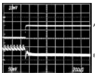
LOAD-TRANSIENT RESPONSE
