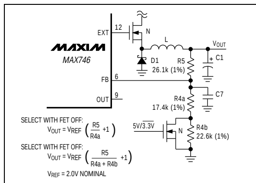
Figure 7. 3.3V/5V Adjustable Output Circuit
