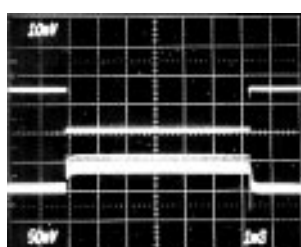
LOAD-TRANSIENT RESPONSE
