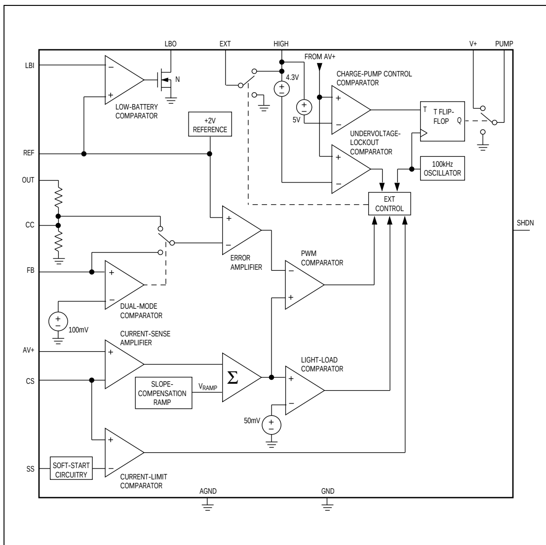
Figure 2. Block Diagram
