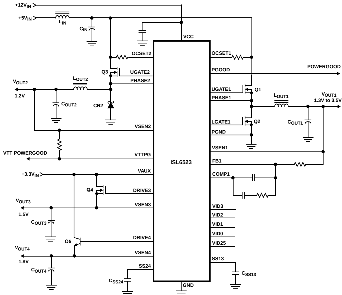
FIGURE 3. TYPICAL APPLICATION
