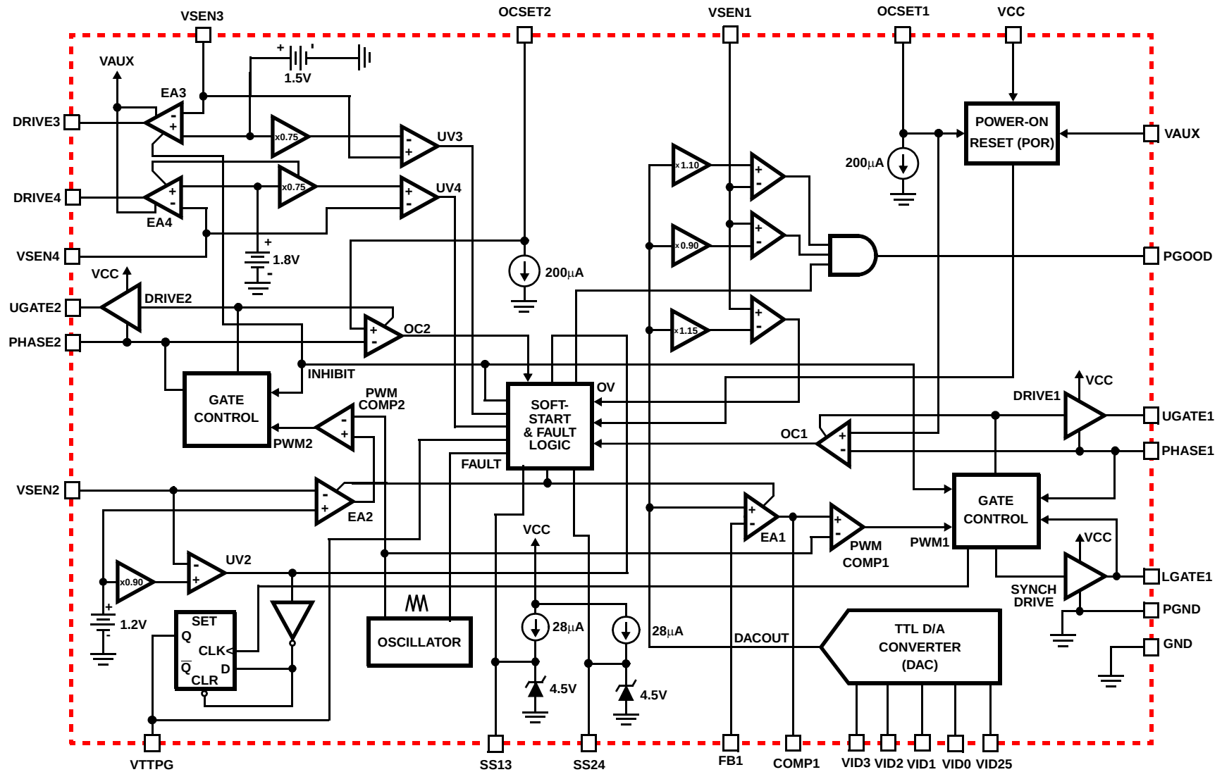
FIGURE 1. BLOCK DIAGRAM
