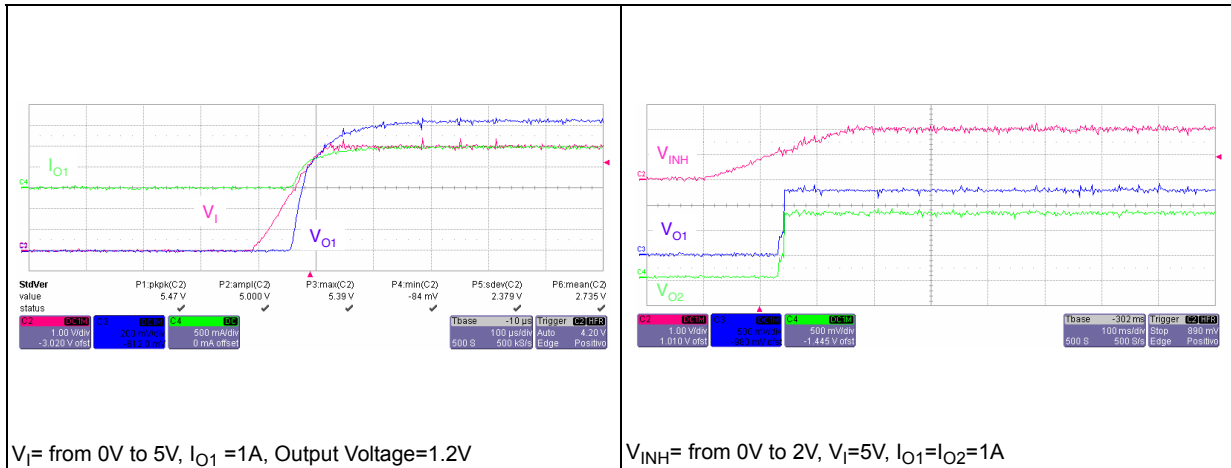
Figure 22. Inhibit transient (ST2S06B)
