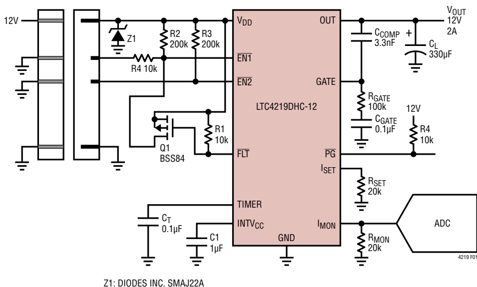
Figure 1. 2A, 12V Card Resident Application with Auto-Retry
