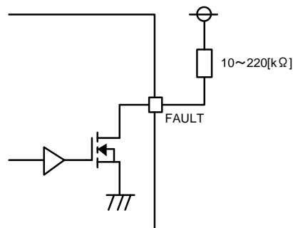
Figure 43. FAULT Terminal
