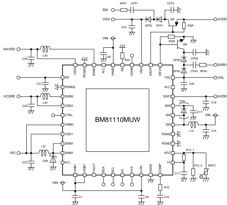
Figure 40. Example Application
