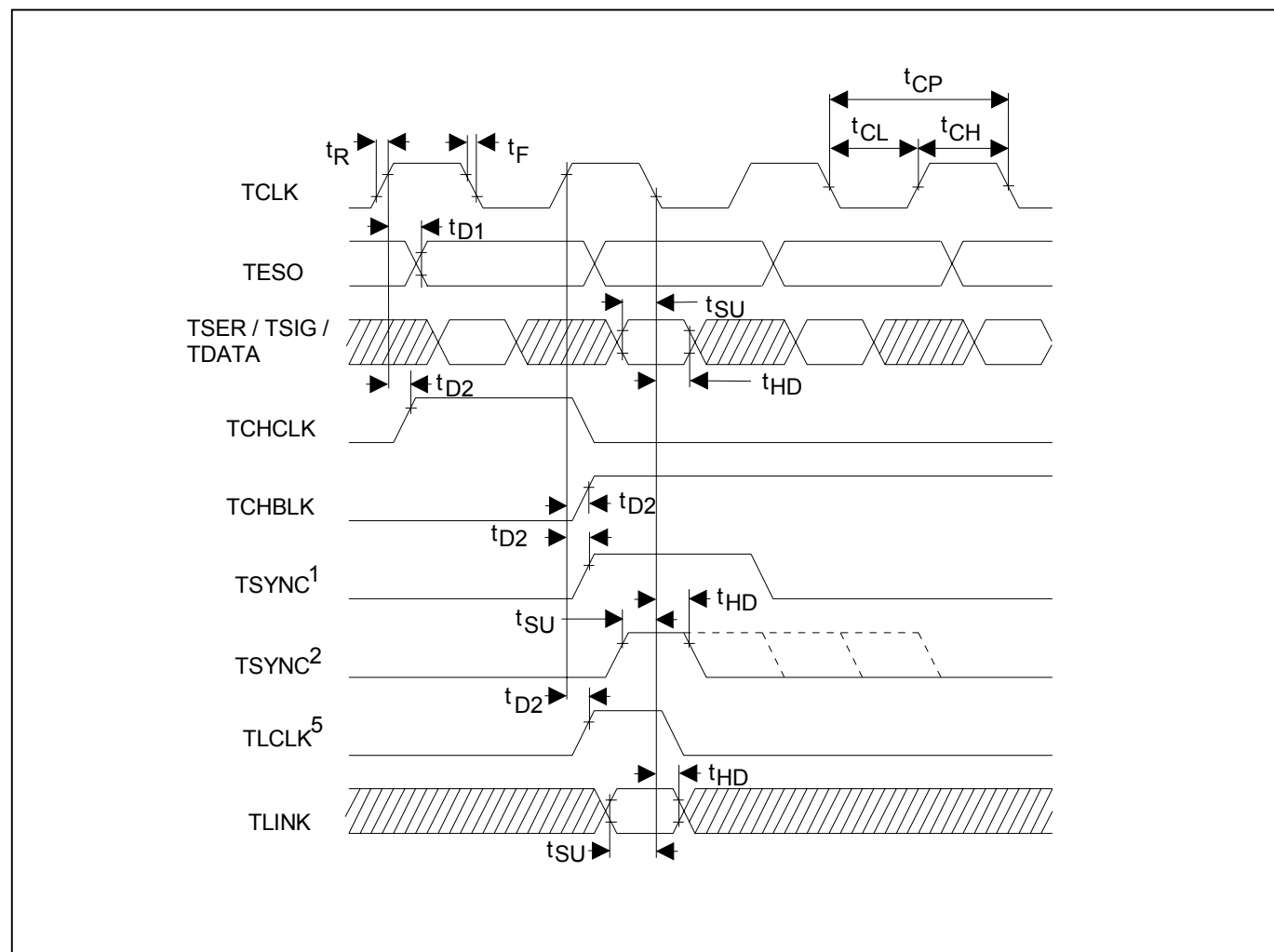
Figure 36-11. Transmit-Side Timing
