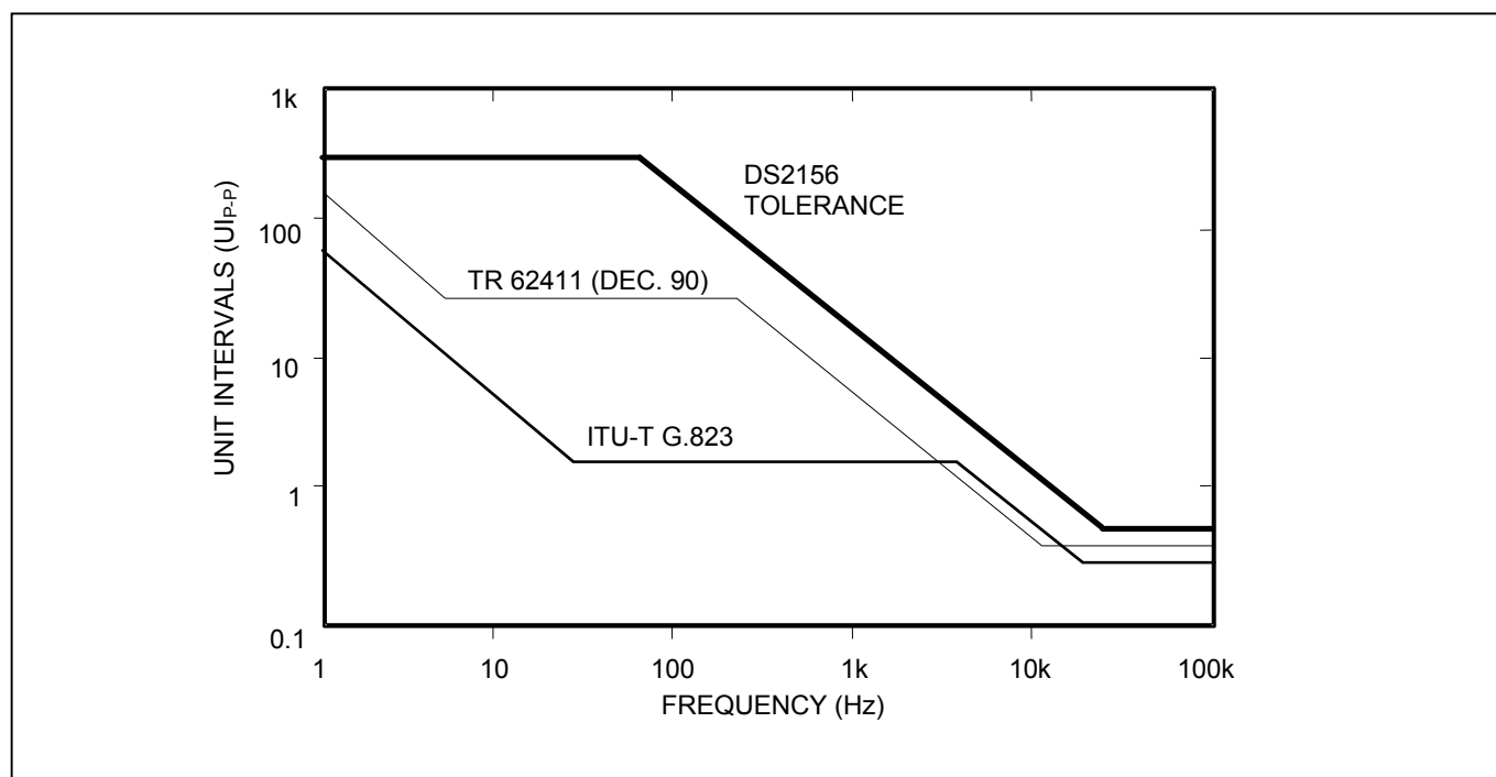
Figure 23-7. Jitter Tolerance
