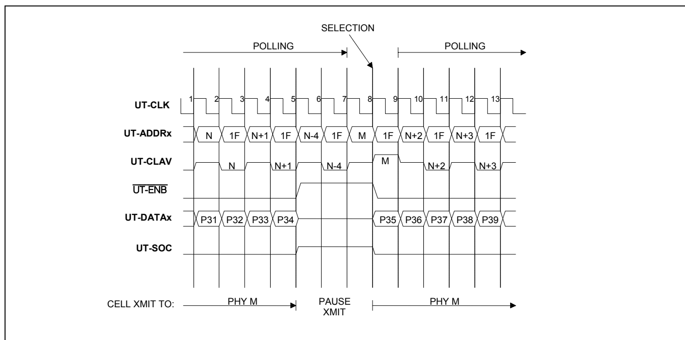
Figure 24-4. Transmission to PHY Paused for Three Cycles
