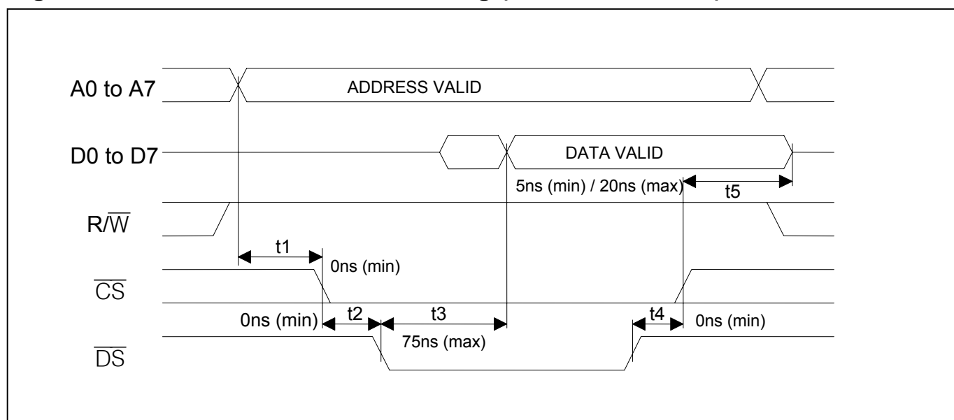
Figure 36-6. Motorola Bus Read Timing (BTS = 1/MUX = 0)
