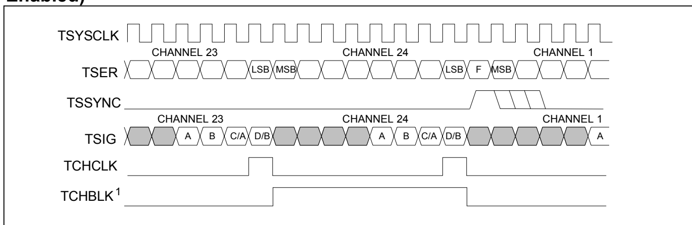
Figure 34-9. Transmit-Side 1.544MHz Boundary Timing (with Elastic Store Enabled)
