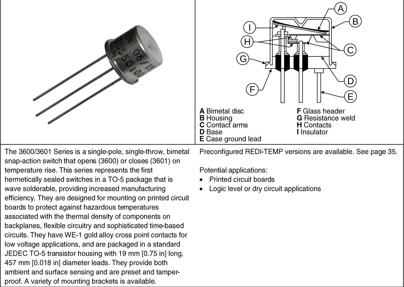
Figure 3. 3600/3601 Series TO-5 Thermal Switches
