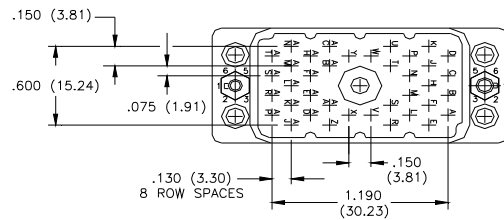
56 PIN PLUG
