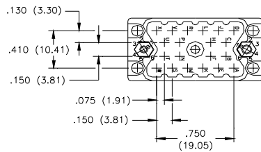
20 PIN PLUG
