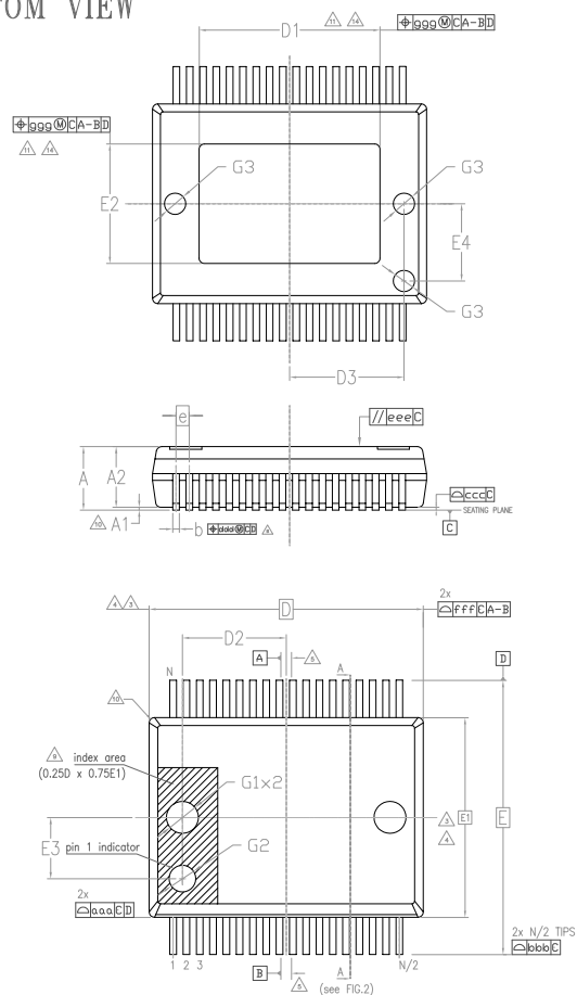
Figure 17. PowerSSO-36 EPD package outline
