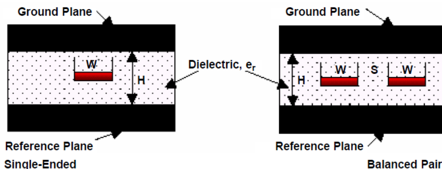
Figure 21. Stripline Topology
