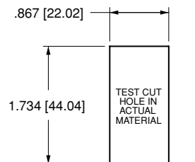
MOUNTING HOLE
