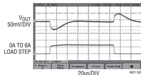
3.3V Transient Response
