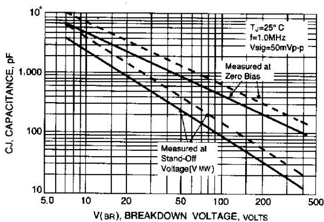
Fig. 4-TYPICAL JUNCTION CAPACITANCE
