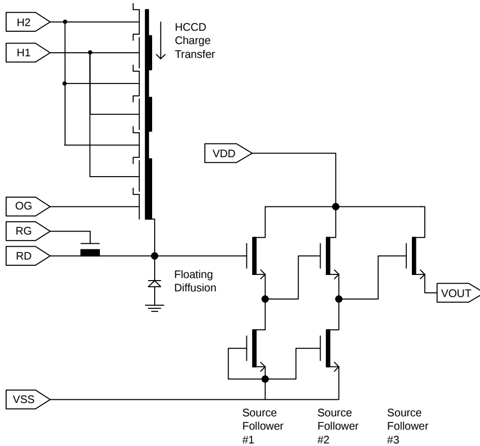
Figure 3. Output Architecture
