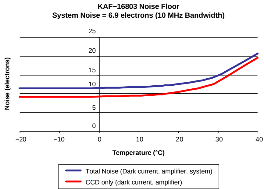
Figure 9. Noise Floor
