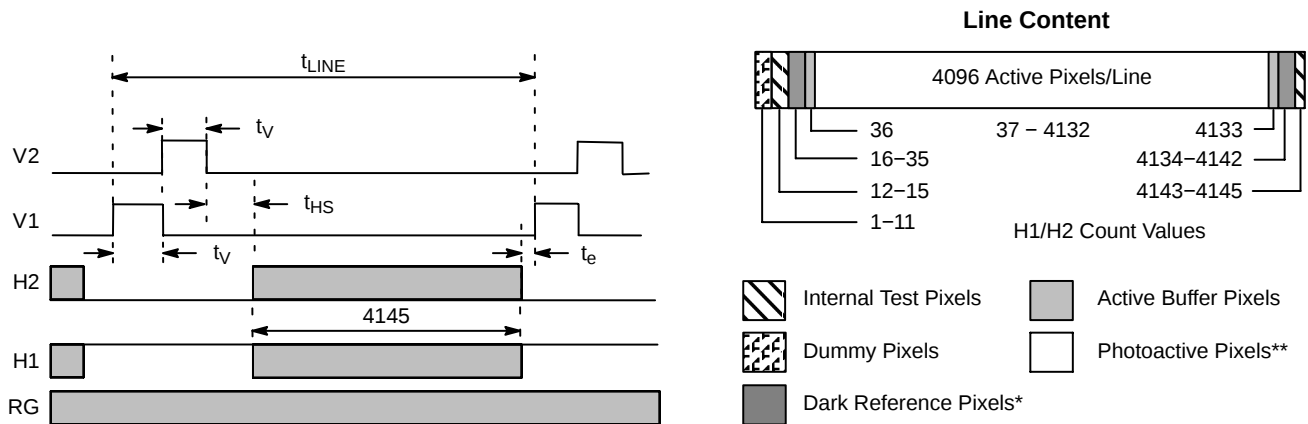
Figure 14. Line Timing
