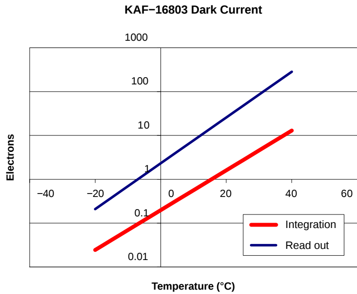
Figure 8. Dark Current
