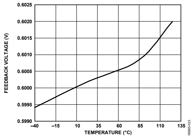
Figure 16. Feedback Voltage vs. Temperature, V_{IN} = 12\text{ V}
