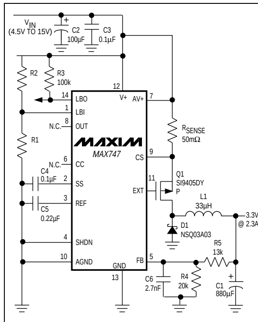
Figure 1b. +3.3V Standard Application Circuit
