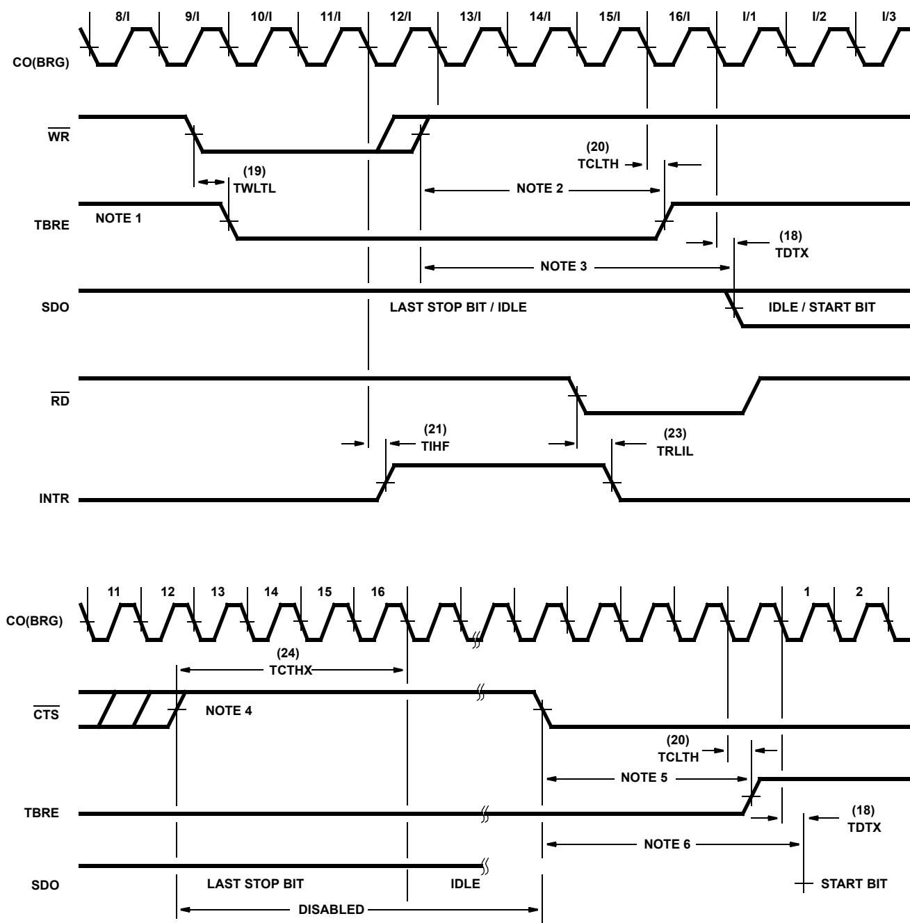
FIGURE 18. TRANSMIT TIMING
