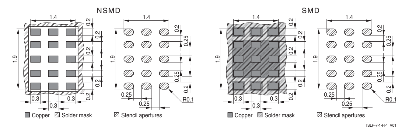
Figure 8-2 Package Footprint
