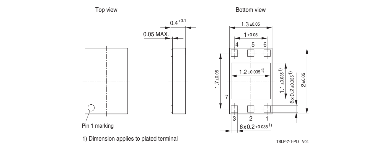
Figure 8-1 Package Outline
