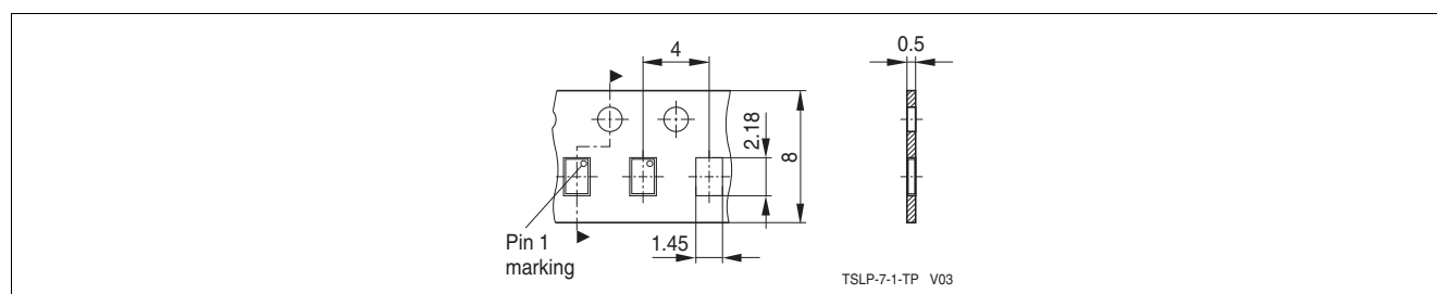
Figure 8-4 Tape Dimensions
