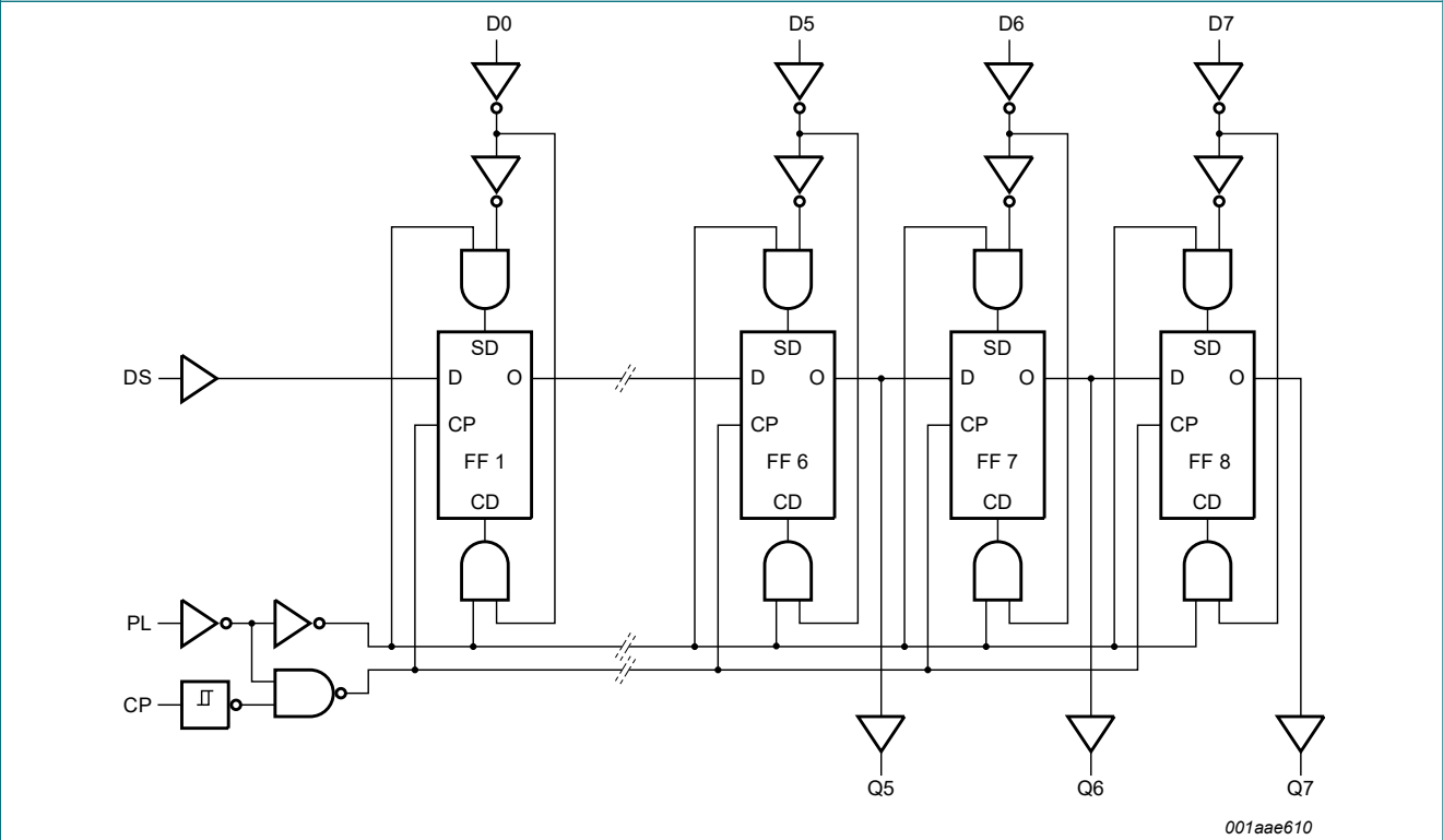
Fig. 2. Logic diagram
