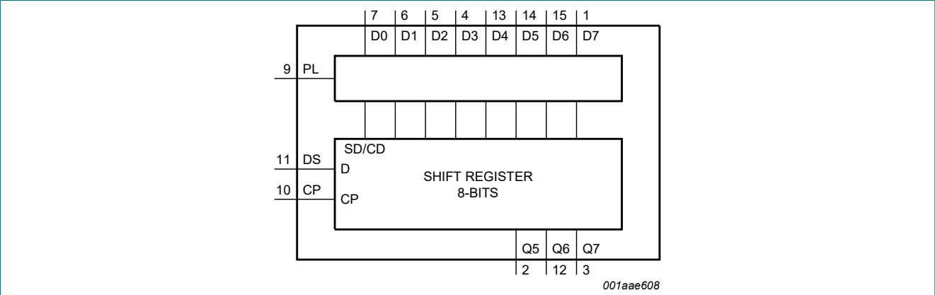
Fig. 1. Functional diagram
