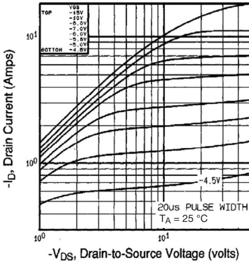
Fig. 1 - Typical Output Characteristics, T_A = 25^\circ C
