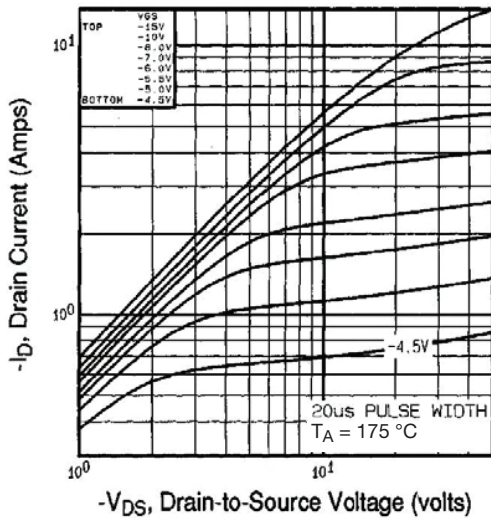
Fig. 2 - Typical Output Characteristics, T_A = 175^\circ C
