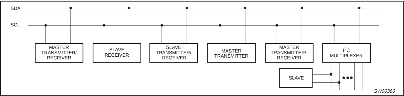
Figure 10. System configuration
