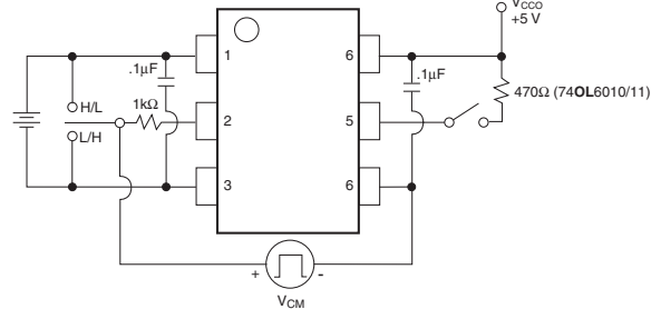
Figure 16. Common Mode Rejection Test Circuit
