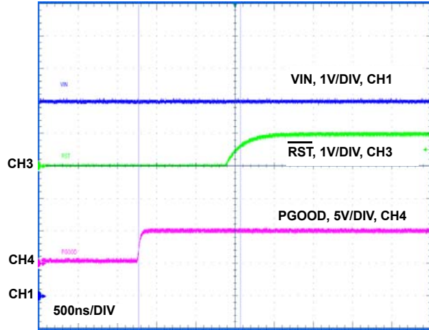
FIGURE 12. PGOOD RISING TO \overline{RST} RISING
