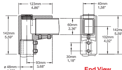
Section of Elbow
