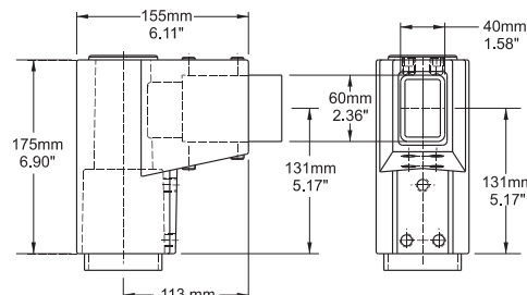
Front View of Elbow
