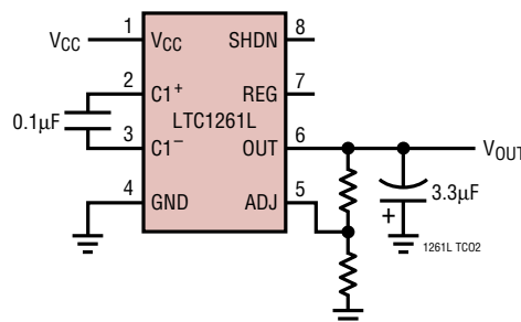
Adjustable Output
