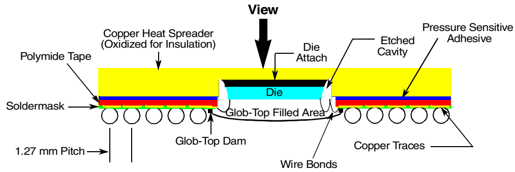
Figure 14. Side View of the TBGA Package
