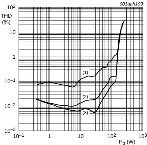
V_P = \pm 27\text{ V} ; double coils; C = 680\text{ nF} . (1) f = 10\text{ kHz} . (2) f = 1\text{ kHz} . (3) f = 100\text{ Hz} . a. R_L = 8\ \Omega
