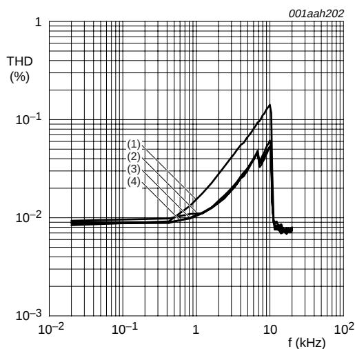
Fig 14. Total harmonic distortion as a function of frequency, SE application with 2 Ω load
