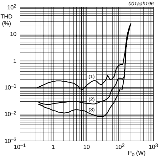
V_P = \pm 27\text{ V} ; double coils; C = 680\text{ nF} . (1) f = 10\text{ kHz} . (2) f = 1\text{ kHz} . (3) f = 100\text{ Hz} . b. R_L = 2\ \Omega .
