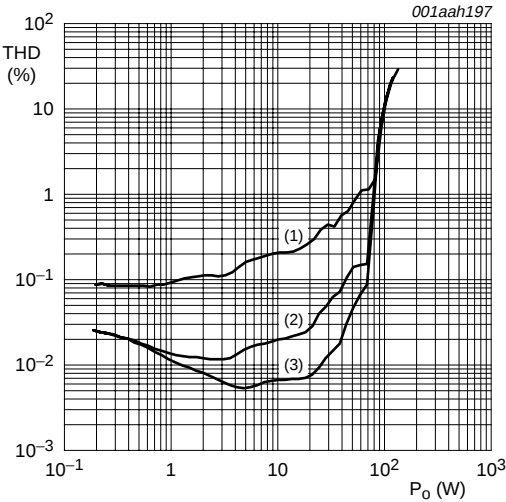
V_P = \pm 27\text{ V} ; double coils; C = 680\text{ nF} . (1) f = 10\text{ kHz} . (2) f = 1\text{ kHz} . (3) f = 100\text{ Hz} . a. R_L = 4\ \Omega .
