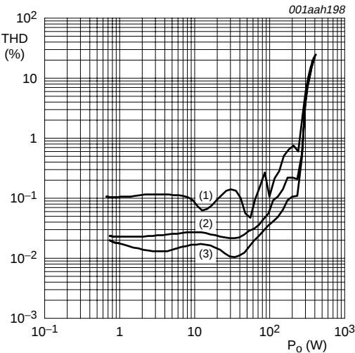
V_P = \pm 27\text{ V} ; double coils; C = 680\text{ nF} . (1) f = 10\text{ kHz} . (2) f = 1\text{ kHz} . (3) f = 100\text{ Hz} . b. R_L = 4\ \Omega
