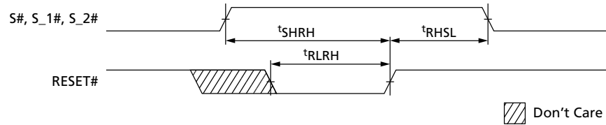
Figure 47: Reset AC Timing During PROGRAM or ERASE Cycle
