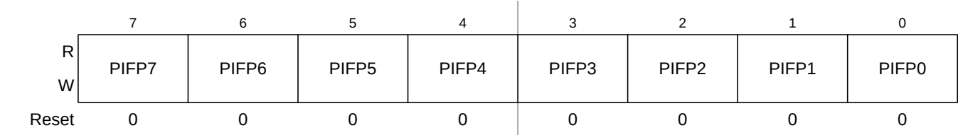
Figure 22-47. Port P Interrupt Flag Register (PIFP)
