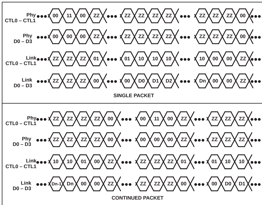
Figure 4–44. Transmit Timing
