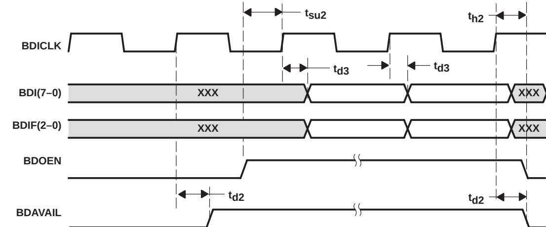
Figure 4–11. Functional Timing for Read Operations in Unidirectional Mode
