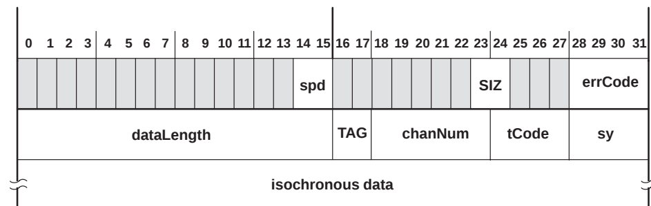
Figure 3–29. Isochronous-Receive Format for Bulky Data FIFO
