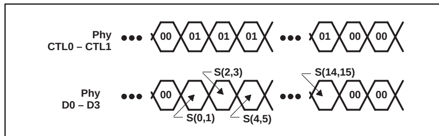
Figure 4-42. LREQ Timing
