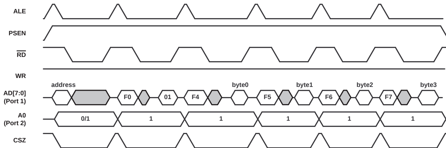
Figure 4–34. Intel 8051 Read Timing (Blind Access Read)
