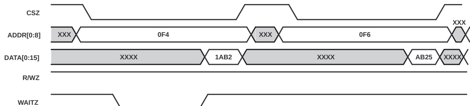
Figure 4–24. TMS320AV7100 Handshake Mode Read Timing
