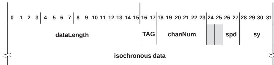
Figure 3–28. Isochronous-Transmit Format
