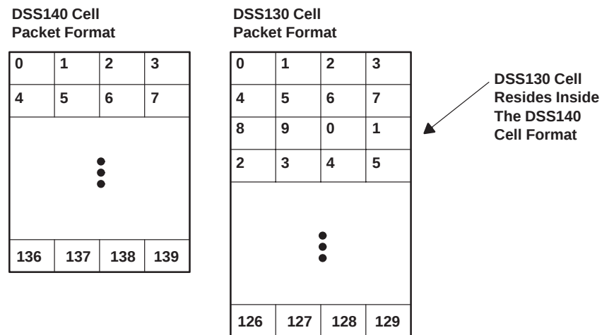
Figure 3–14. DSS130 Packets
