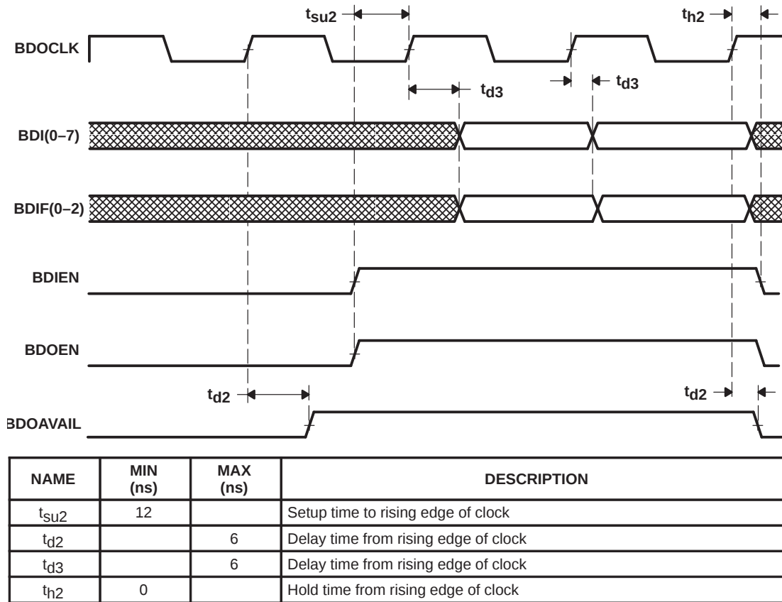
Figure 4-17. Critical Timing for Read Operations in Bidirectional Mode
