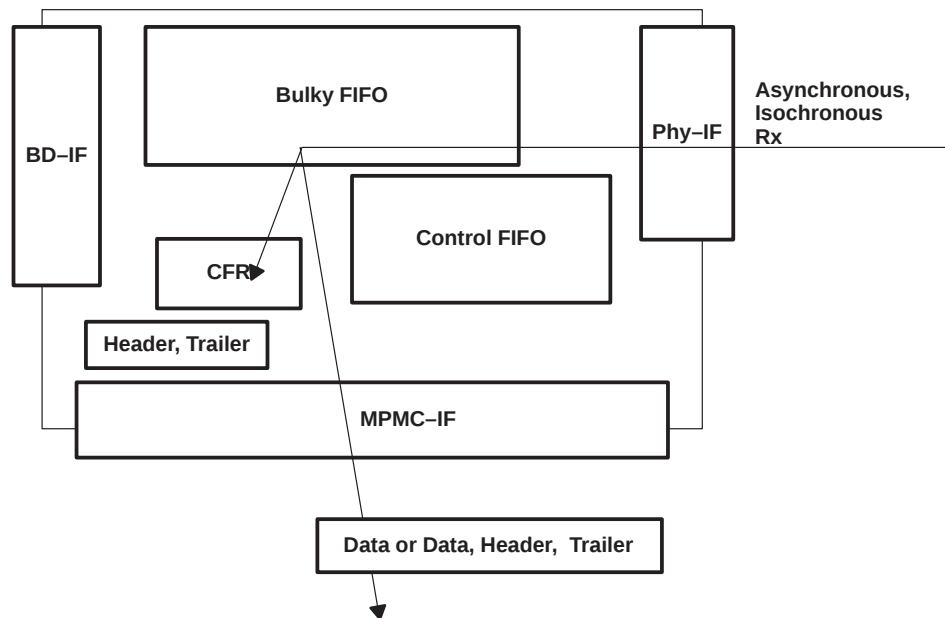
Figure 3–16. Receive Asynchronous/Isochronous Data to Microprocessor Interface
