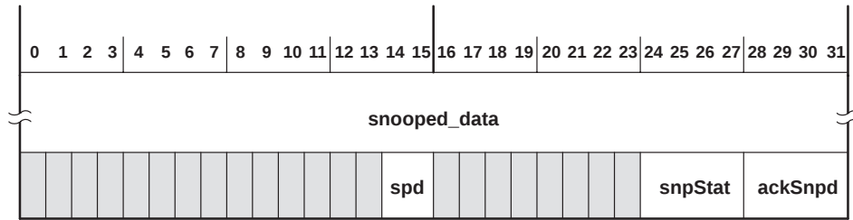
Figure 3–30. Snoop Format
