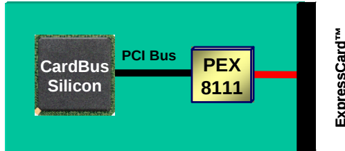
Figure 2. Forward Bridge in ExpressCard™
