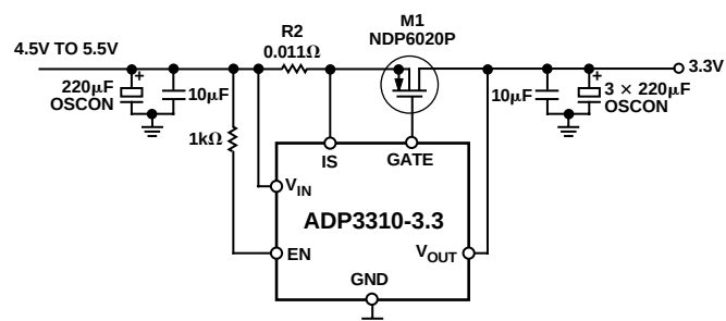
Figure 14. Typical 3 A Low Dropout Regulator Circuit
