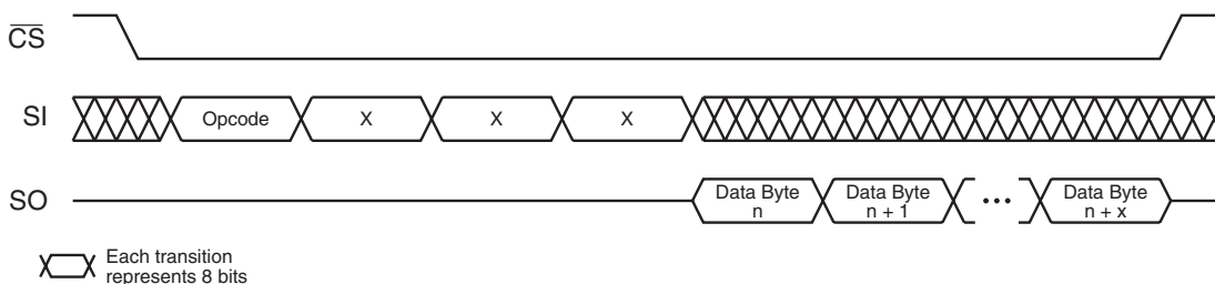
Figure 10-4. Read Security Register
