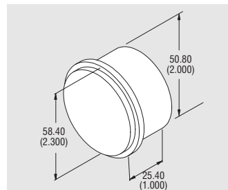
Panel Cutout: 52.3 (2.060) Approximate in mm (inches).
