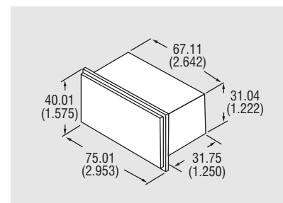
Panel Cutout: 33 x 68 mm (1.299 x 2.677) Approximate in mm (inches)
