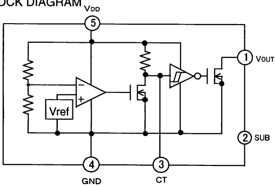
OBLOCK DIAGRAM
