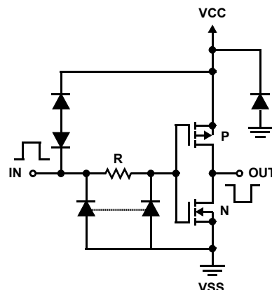
FIGURE 1. SCHEMATIC DIAGRAM, 1 OF 6 IDENTICAL UNITS
