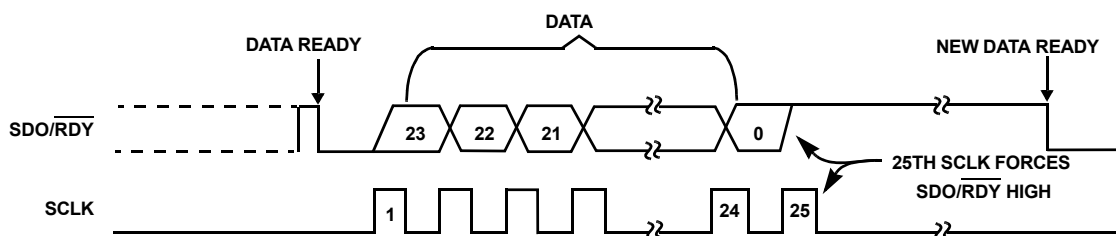
FIGURE 31. OUTPUT DATA WAVEFORMS FOR SDO/ \overline{\text{RDY}} POLLING
