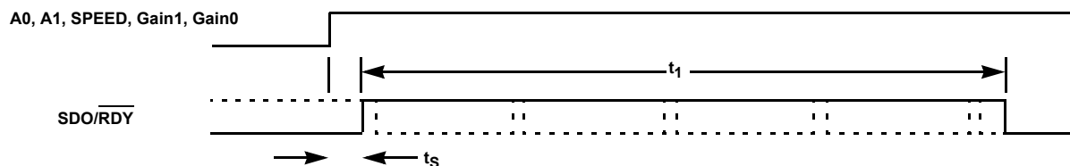
FIGURE 28. SDO/RDY DELAY AFTER MULTIPLEXER CHANGE
