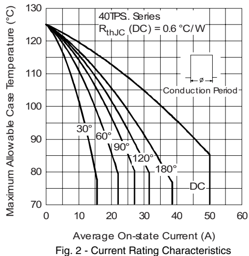
Fig. 2 - Current Rating Characteristics
