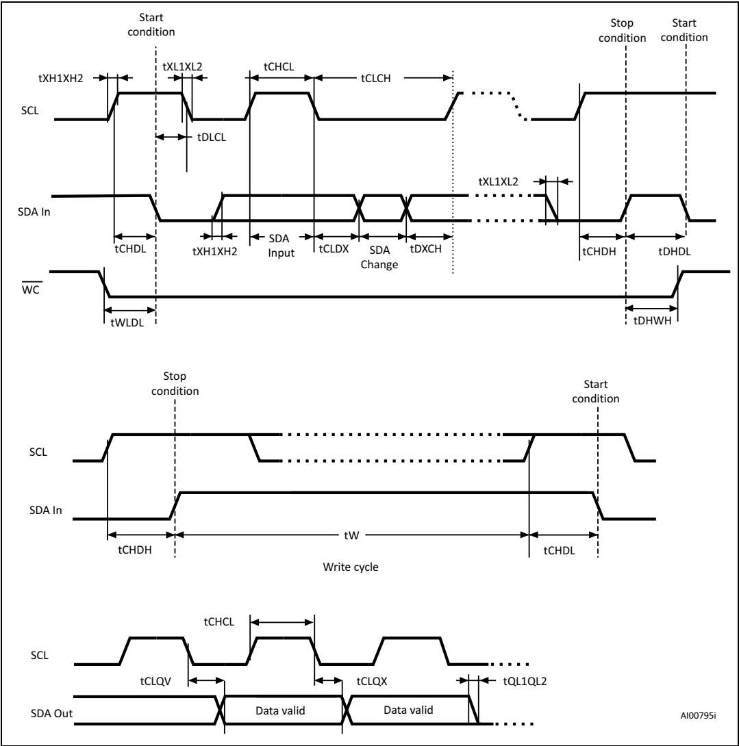
Figure 13. AC waveforms
