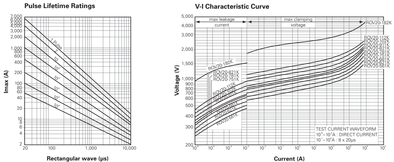
Figure V15 - ROV20-561K-ROV20-182K
