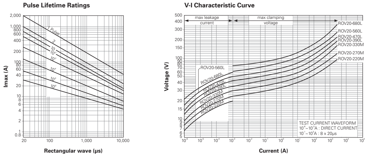
Figure V14 - ROV20-101K-ROV20-511K
