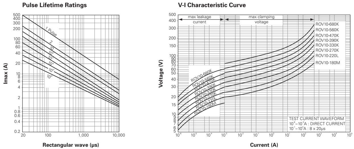
Figure V8 - ROV10-820K~ROV10-511K
