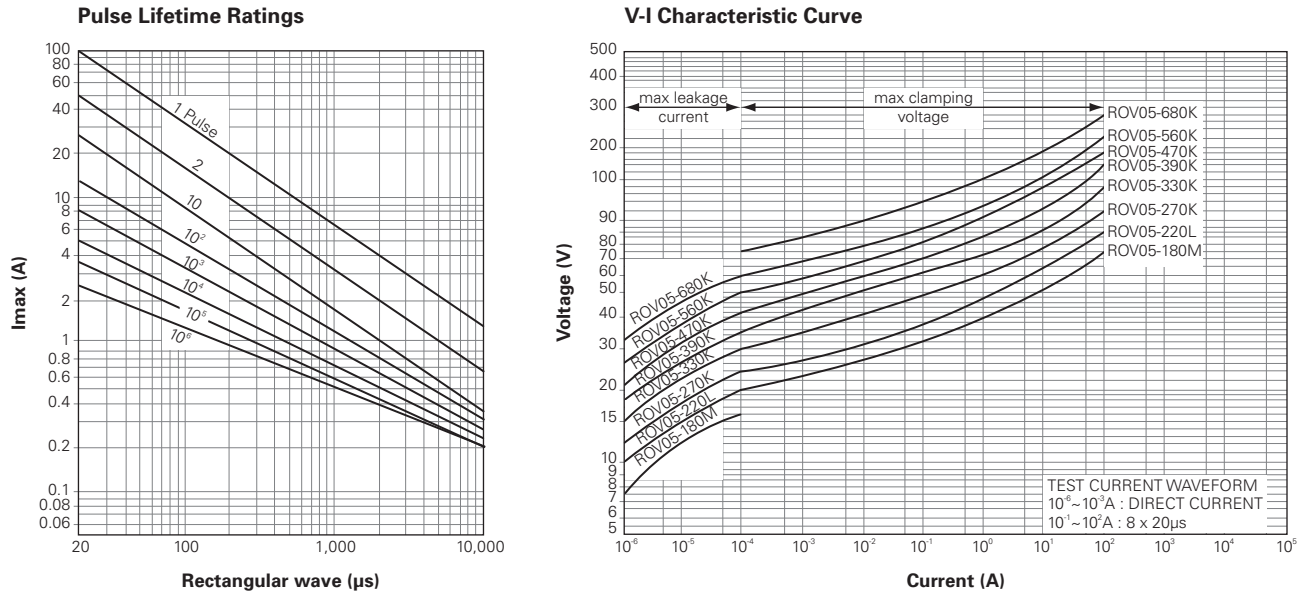
Figure V3 - ROV05-180M-ROV05-680K
