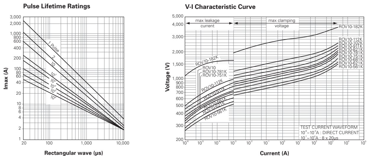
Figure V9 - ROV10-561K~ROV10-182K
