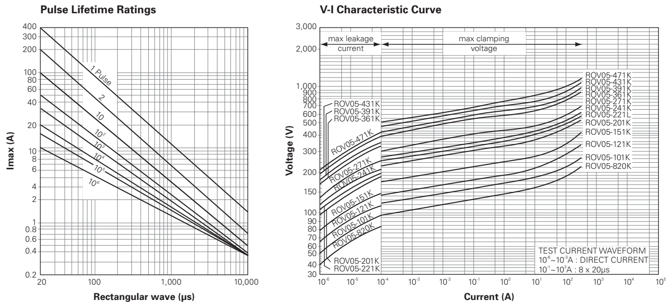
Figure V4 - ROV05-820K-ROV05-471K
