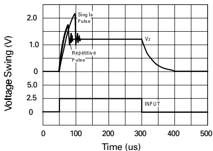
Pulse Response
