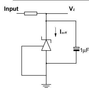
Fig 3 – Test Circuit for Off State current
