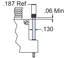
Code E & EJ EJ - Extended Jackscrew E - Extended Screwlock
