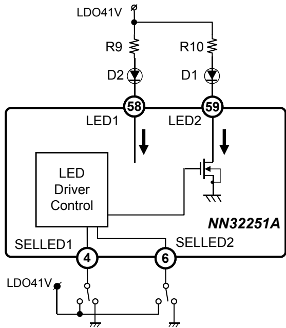
Figure A-4. LED Circuit Diagram
