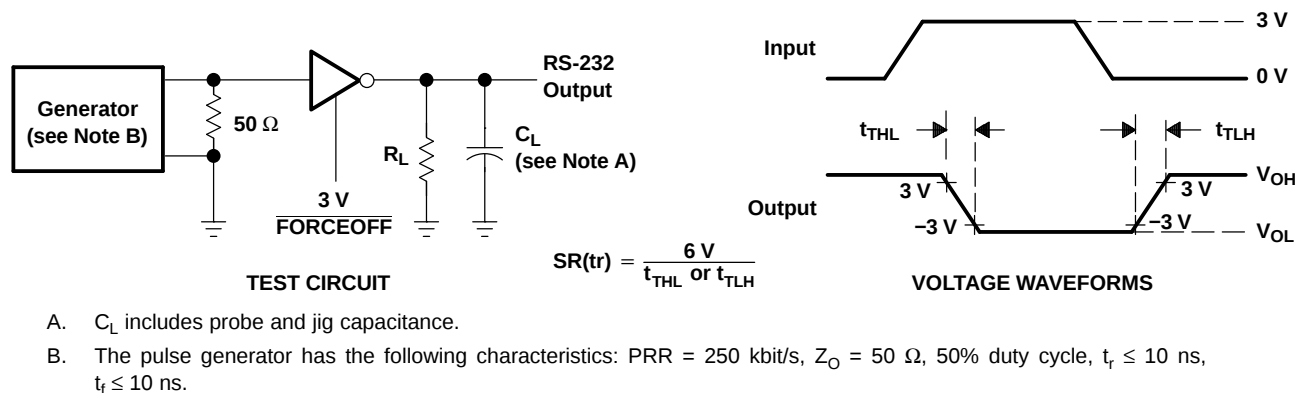
Figure 1. Driver Slew Rate
