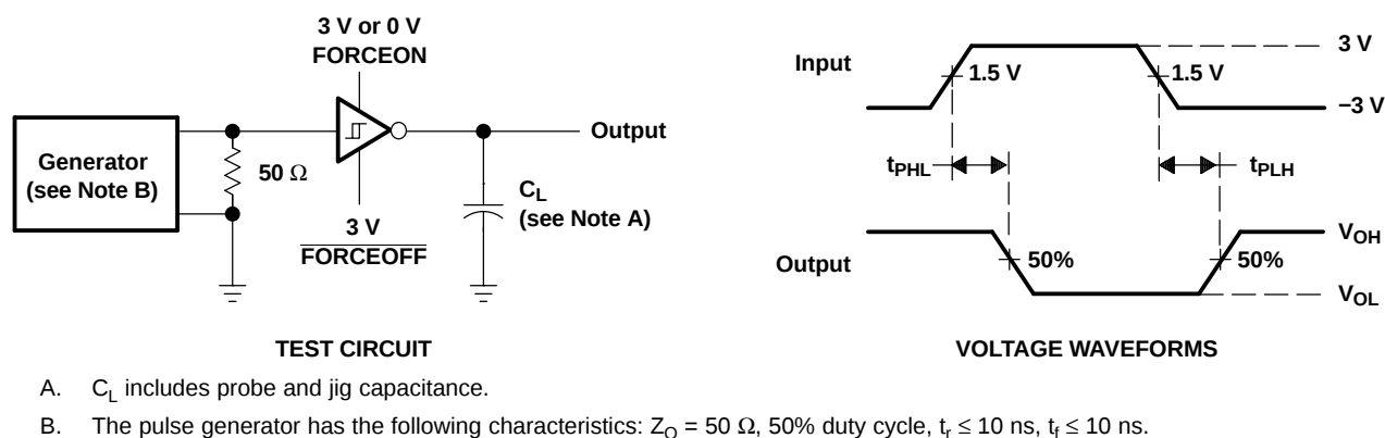
Figure 3. Receiver Propagation Delay Times
