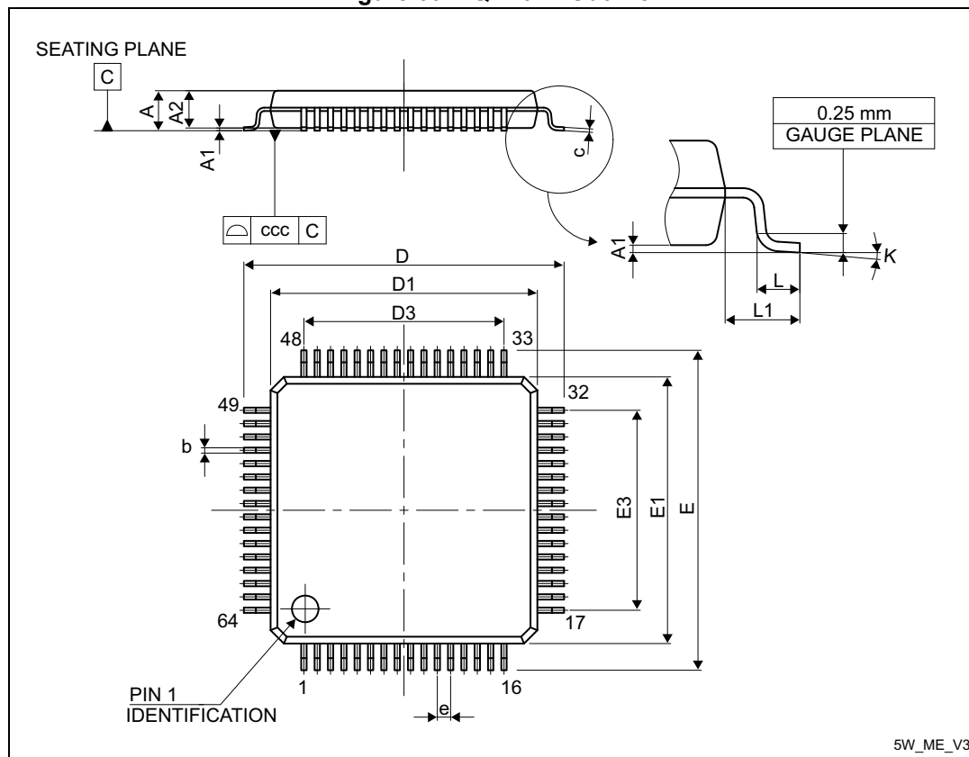
Figure 60. LQFP64 - Outline
