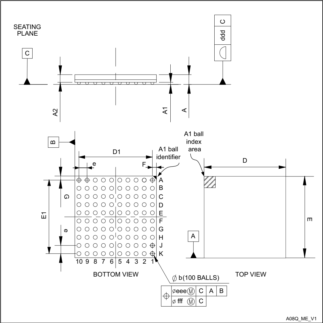
Figure 64. TFBGA100 - Outline
