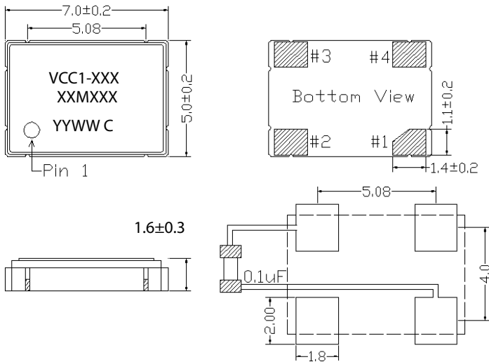
Recommended Soldering Pad Layout
