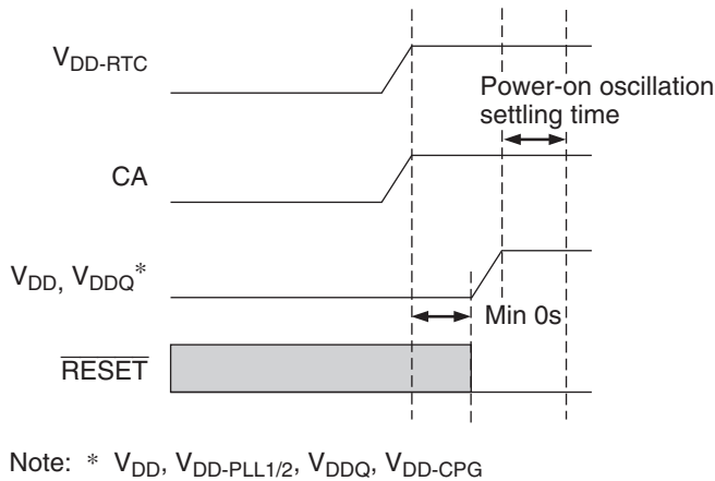
Figure 9.15 Timing When VDD-RTC Power Is Off → On
