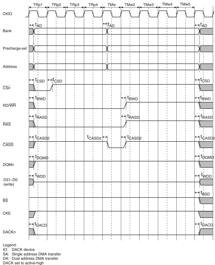
Figure 23.34 (a) Synchronous DRAM Bus Cycle: Mode Register Setting (PALL)
