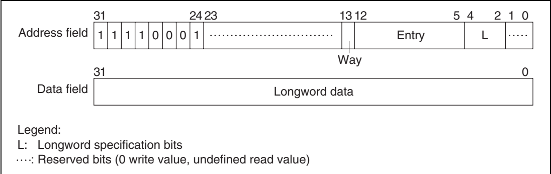
Figure 4.13 Memory-Mapped IC Data Array
