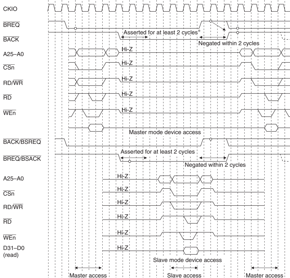
Figure 13.69 Arbitration Sequence
