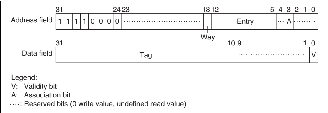
Figure 4.12 Memory-Mapped IC Address Array
