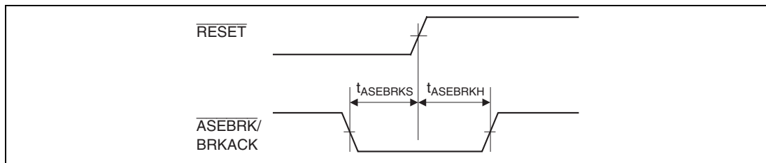
Figure 23.66 RESET Hold Timing
