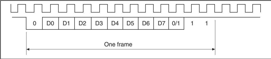
Figure 15.6 Relation between Output Clock and Transfer Data Phase (Asynchronous Mode)
