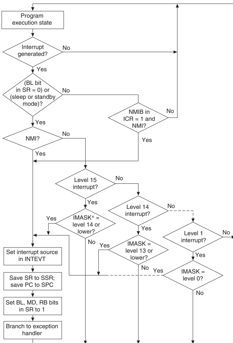
Figure 19.3 Interrupt Operation Flowchart
