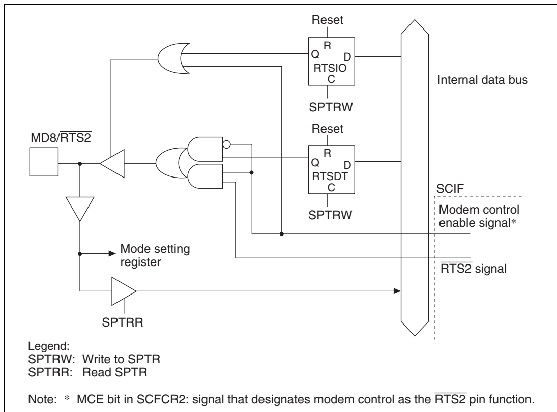
Figure 18.10 MD8/RTS2 Pin
