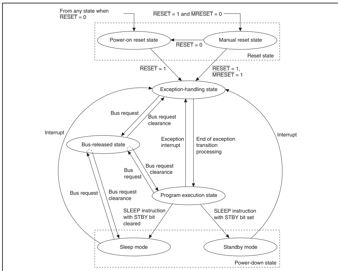
Figure 2.6 Processor State Transitions
