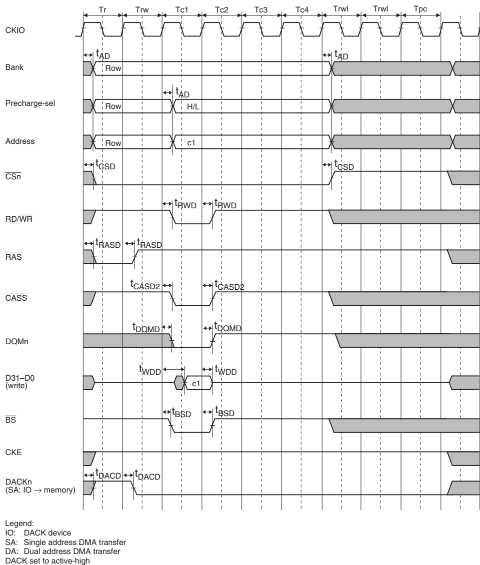
Figure 23.26 Synchronous DRAM Auto-Precharge Write Bus Cycle: Single (RCD [1:0] = 01, TPC [2:0] = 001, TRWL [2:0] = 010)
