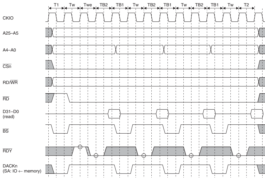
Figure 13.42 Burst ROM Wait Access Timing
