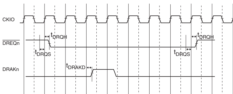
Figure 23.64 (a) \overline{\text{DREQ}} /DRAK Timing
